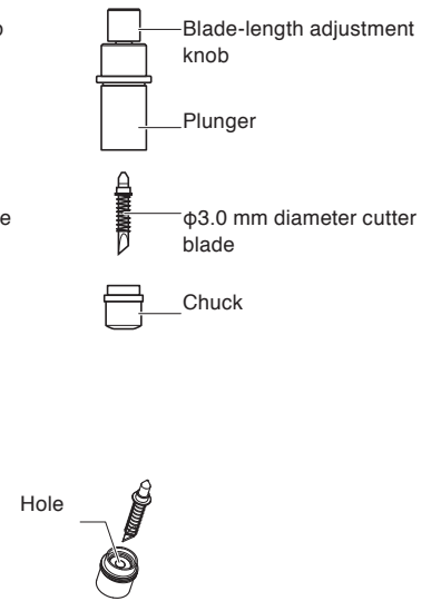
PHP34-CB30-HS φ3.0 mm diameter cutter Plunger
